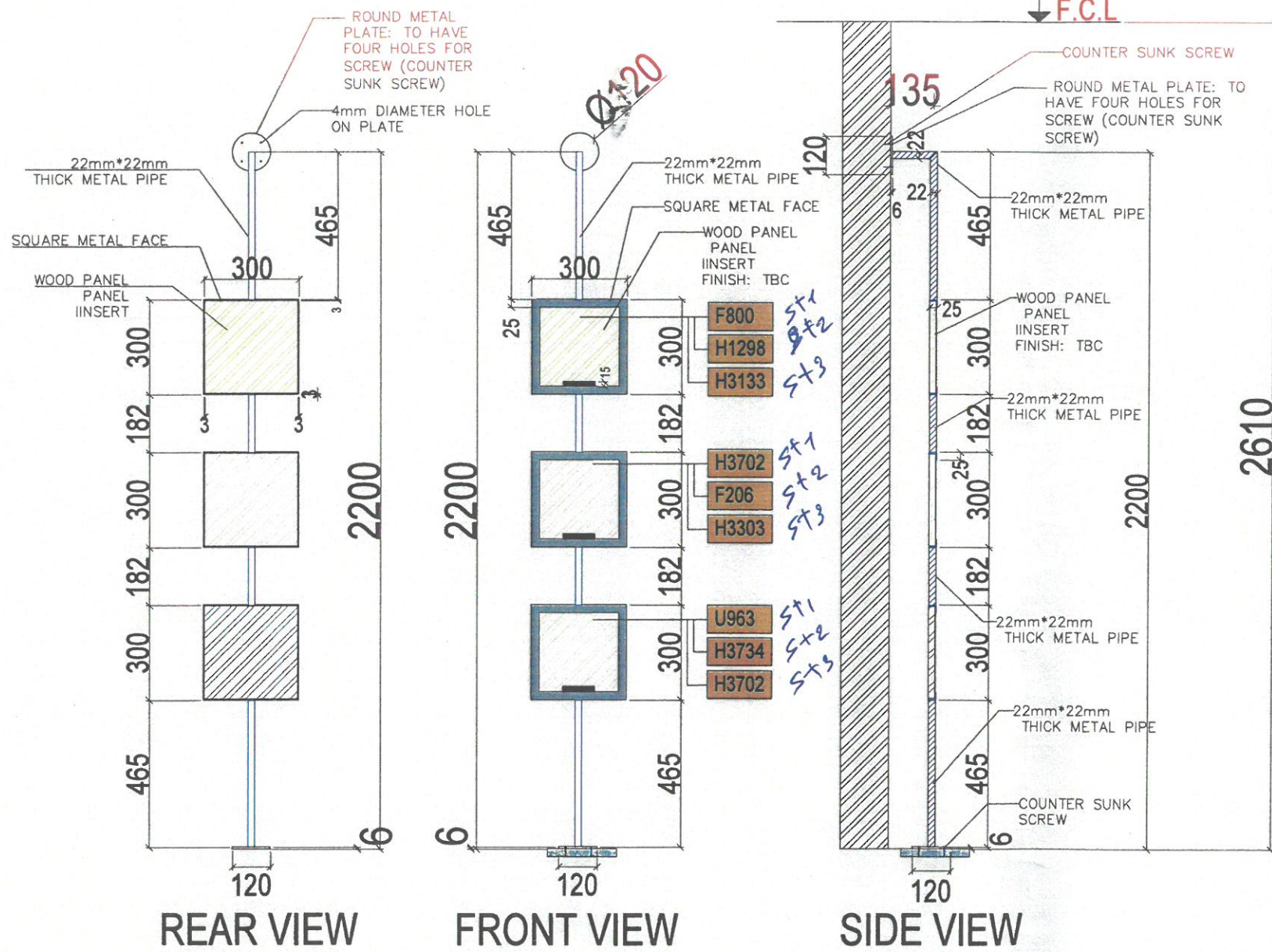
DISPLAY WALL PANEL WITH METAL STAND-(F2)-3 PCS
