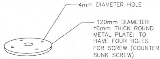
TOP AND BASE METAL PLATE
