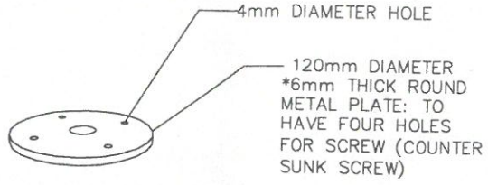
TOP AND BASE METAL PLATE
