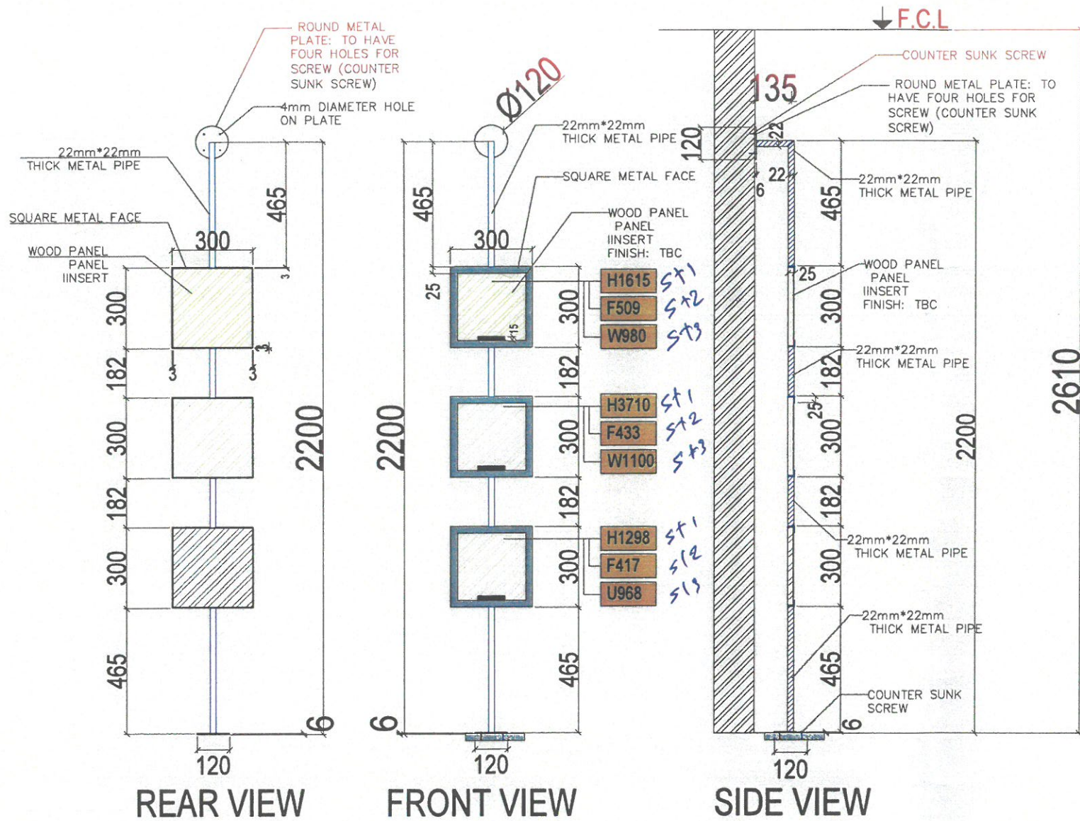
REAR VIEW SQUARE METAL
